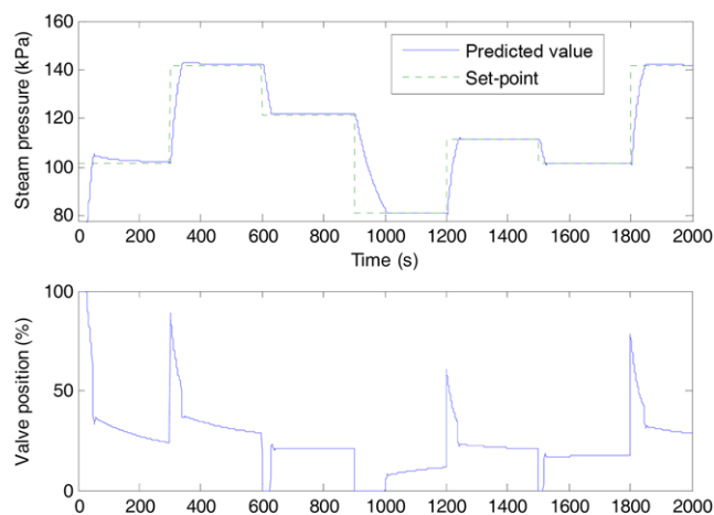
Fig. 9. Results of MPC simulations for the steam pressure.
