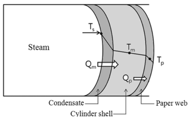
Fig. 1. The temperature profile and the energy flows in the drying cylinder.
